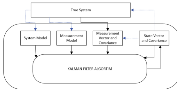
Figure 1: Elements of the Kalman filter (Groves, 2008).
