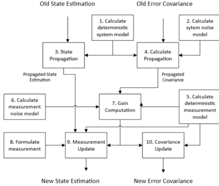
Figure 2: Flow of Kalman Filter
